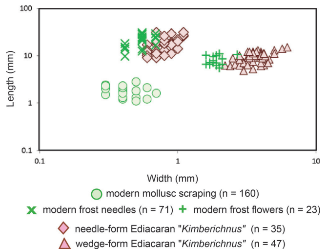
Fig. 10—Measurements of length and width of scratch marks from the radulae of modern marine molluscs (mainly limpets and chitons) on siltstone at Point Loma near San Diego, California (see Dombos et al. , 2004), are very distinct from length and width of frost needles (Fig. 9B) and flowers (Fig. 9A), and comparable fossils from the Ediacara Member of the Rawnsley Quartzite in South Australia, including the needle-morph of “ Kimberichnus ” (South Australian Museum P35663 from Mt Scott) and the wedge-morph of “ Kimberichnus ” (South Australian Museum P35651a from Bathub Gorge, see Gehling et al. , 2014).
