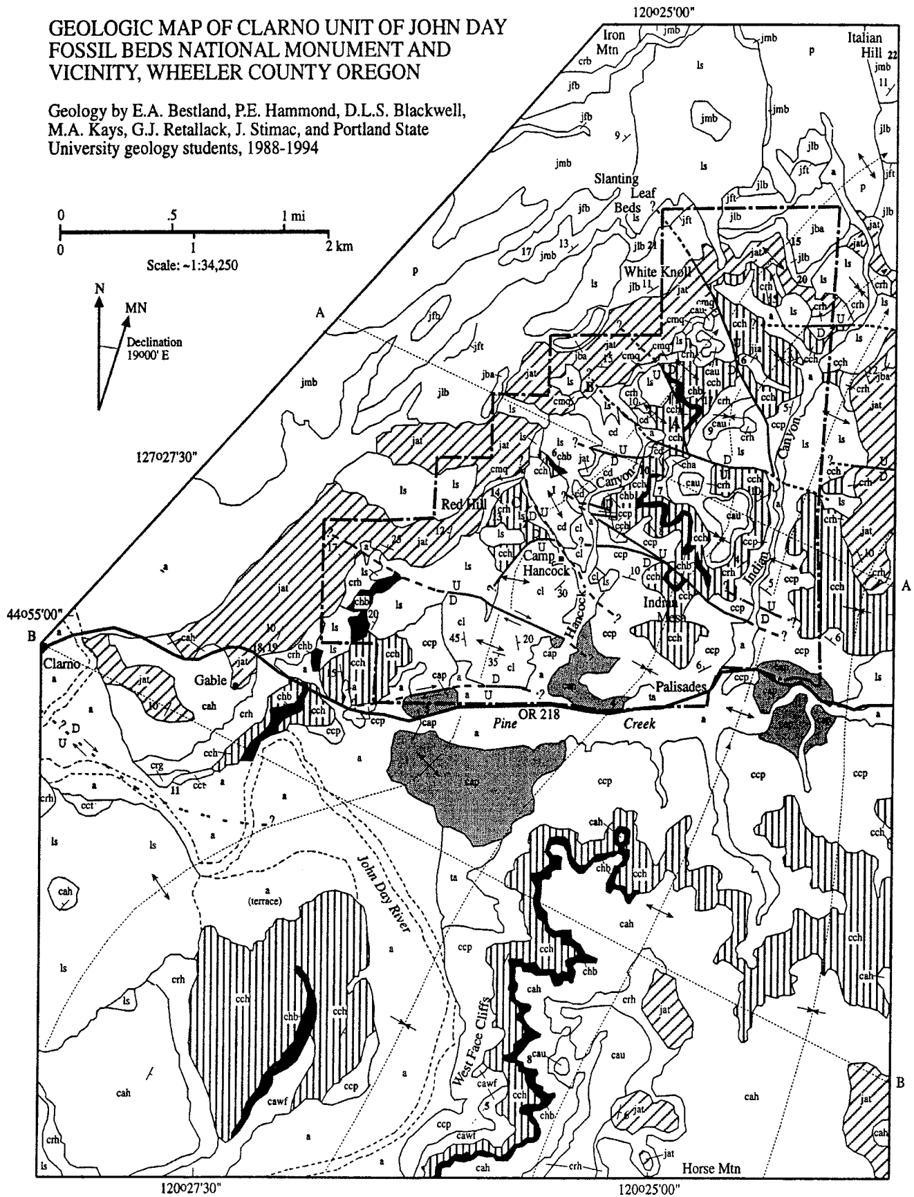
Figure 3. Informal geologic map of the Clarno Unit of the John Day Fossil Beds National Monument and vicinity (modified from Bestland and Retallack, 1994a; unpublished mapping by P.E. Hammond and Portland State University students; and unpublished mapping by M.A. Kays, D.L.S. Blackwell, J. Stimac, and E.A. Bestland).
