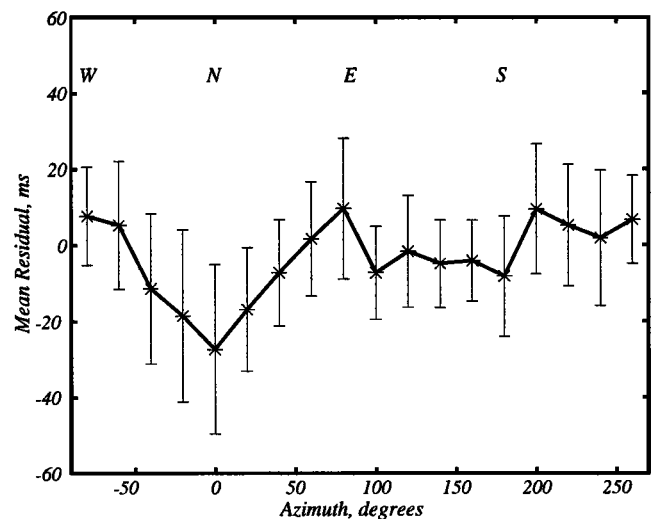
Figure 5. Travel-time residuals (observed minus predicted) for the three-dimensional inversion of Figure 4 averaged in 20° azimuth bins and plotted against the source-receiver azimuth. The azimuth is calculated relative to the orientation of the ridge axis. Error bars show the standard deviation of the residuals (not the standard deviation of the mean).
