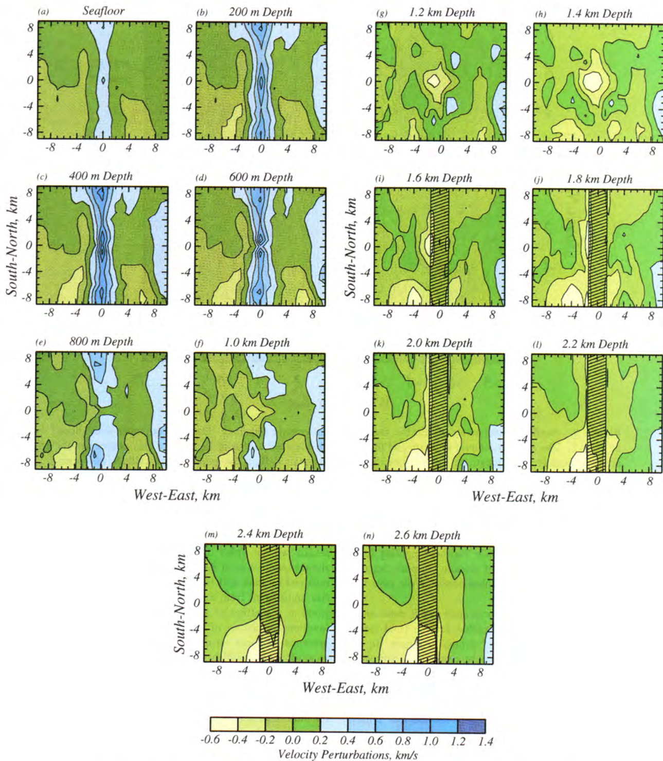
Plate 1. Results of a three-dimensional inversion; the initial model is the two-dimensional starting model shown in Figure 6a. (a)-(n) Map view sections of the anomalous velocity perturbations relative to the prior model. Sections are shown at 200-m intervals from the seafloor down to 2.6 km depth. Except for the hachured region, the velocity of the prior model at the depth of each section is as follows: (a) 1.9 km/s, (b) 3.9 km/s, (c) 4.4 km/s, (d) 5.0 km/s, (e) 5.4 km/s, (f) 5.7 km/s, (g) 6.1 km/s, (h) 6.4 km/s, (i) 6.5 km/s, (j) 6.7 km/s, (k)-(n) 6.8 km/s. The contour interval is 0.2 km/s. Hachured area at depths of 1.6-2.6 km delimits approximate location of axial magma chamber anomaly included in the starting model. See text for discussion.
