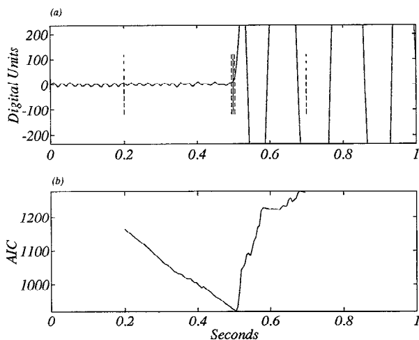
Figure 2. An example of the automated identification of the P wave onset and arrival time uncertainty. (a) Seismogram recorded by an ocean bottom receiver at a range of 10 km. Dashed lines indicate data window used to evaluate the autoregressive models; solid vertical line indicates automated pick; dotted vertical lines show the estimated standard deviation in the arrival time. Note the impulsiveness of the P wave arrival, which is typical of data used in the current analysis. The zero point of the time axis is arbitrary. (b) A plot of the Akaike Information Criterion (AIC [Takanami and Kitagawa, 1988]) as calculated by the autoregressive method; see text for details. The minimum in the AIC defines the P wave onset.
