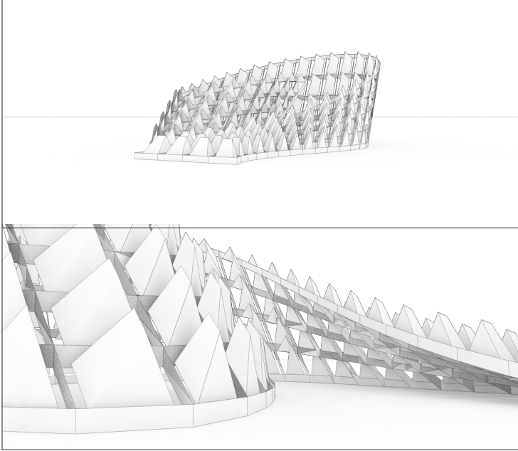
SPRING EQUINOX
