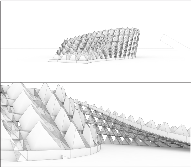
SUMMER SOLSTICE
