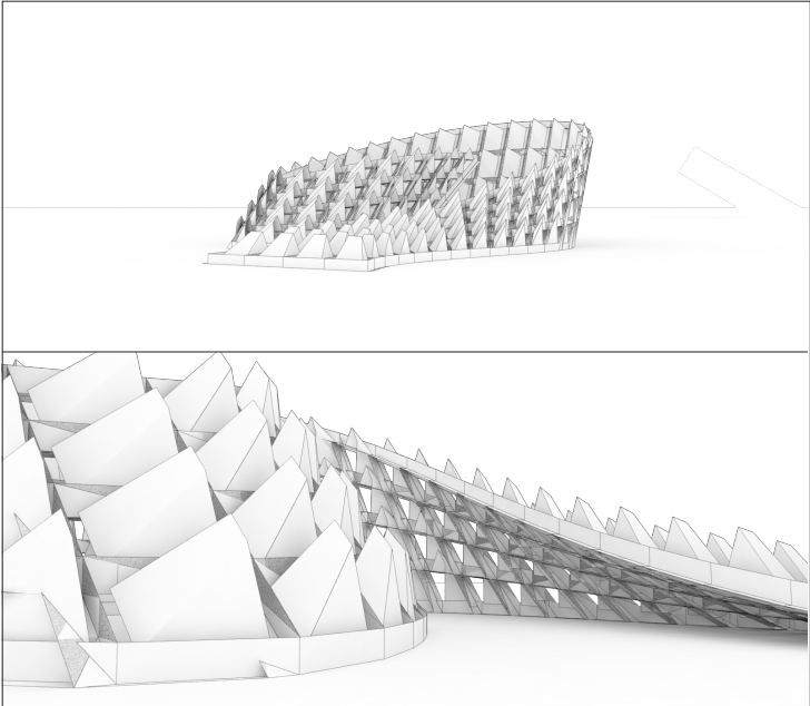
SUMMER SOLSTICE
