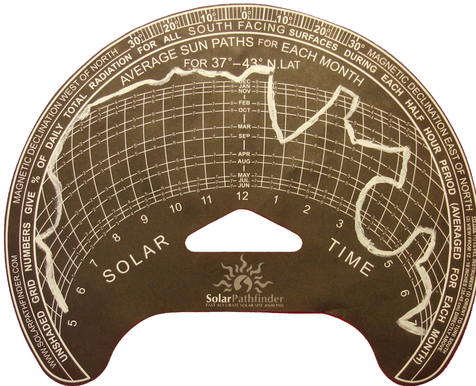
Site Tracing on a Monthly Sunpath Diagram
